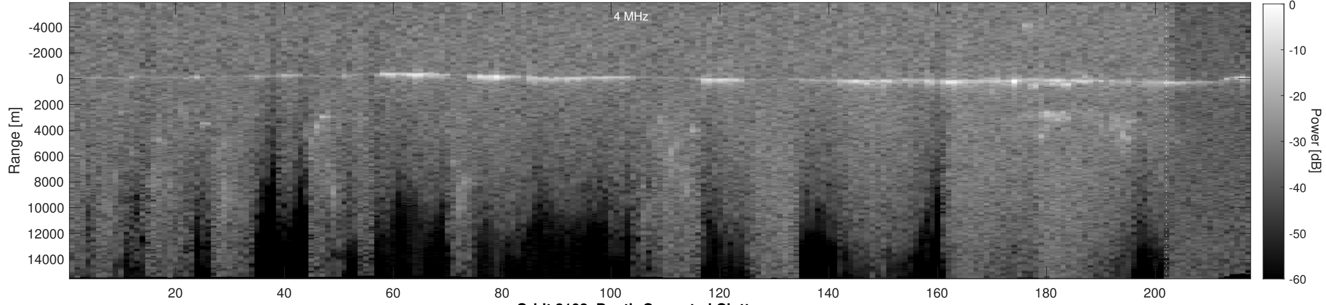
Orbit 3192, Depth-Corrected Cluttergram
