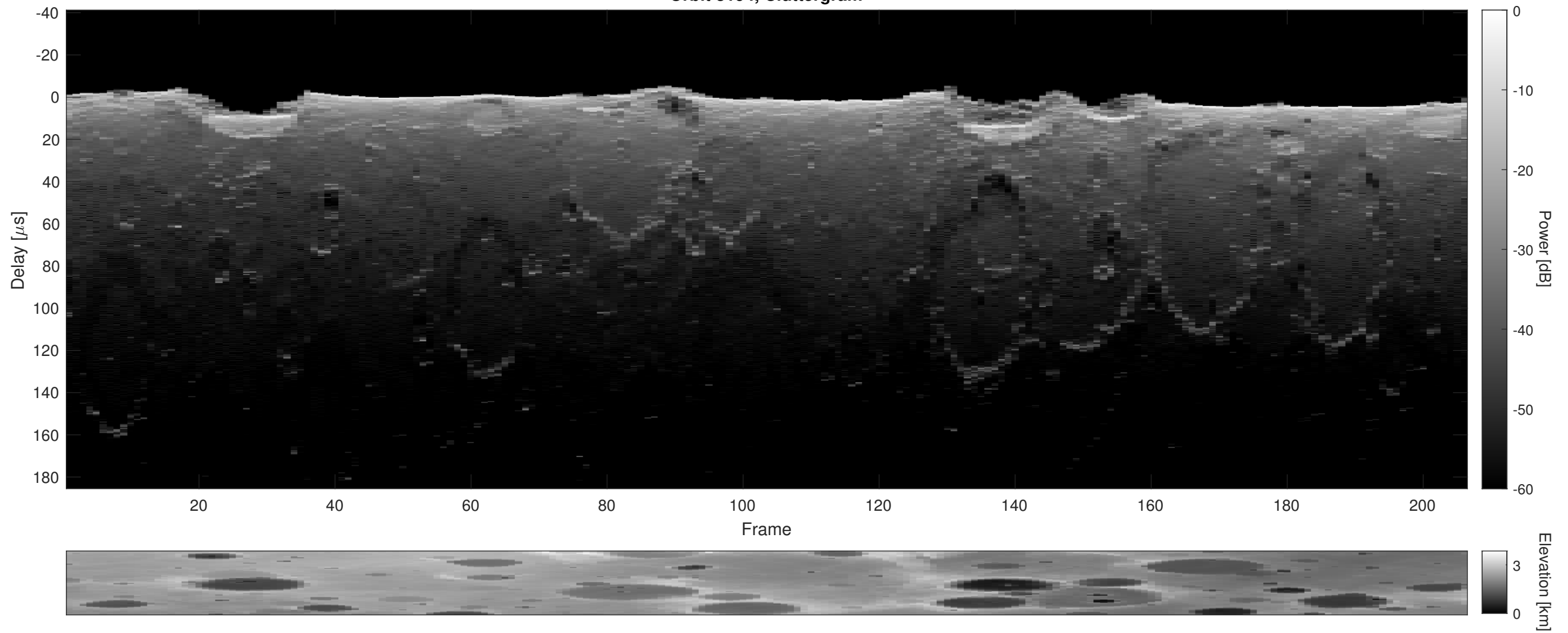
Orbit 3194, Cluttergram
