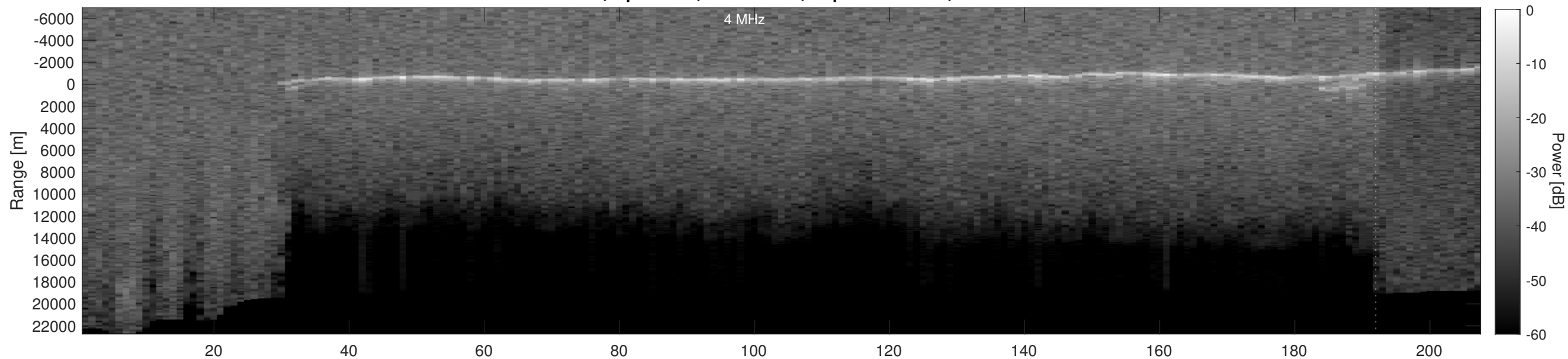
Orbit 3195, Depth-Corrected Cluttergram
