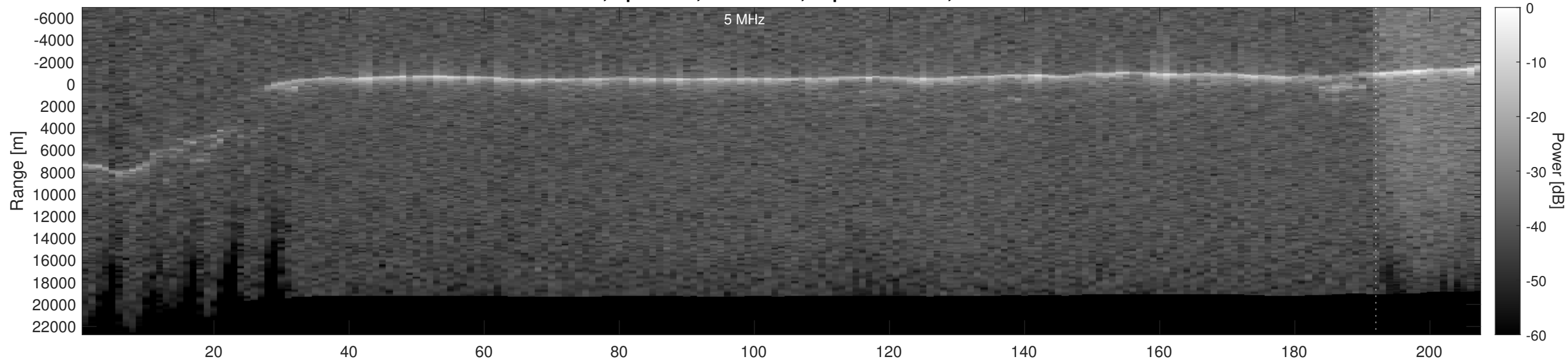
Orbit 3195, Optimized, No Window, Depth-Corrected, Channel 2
