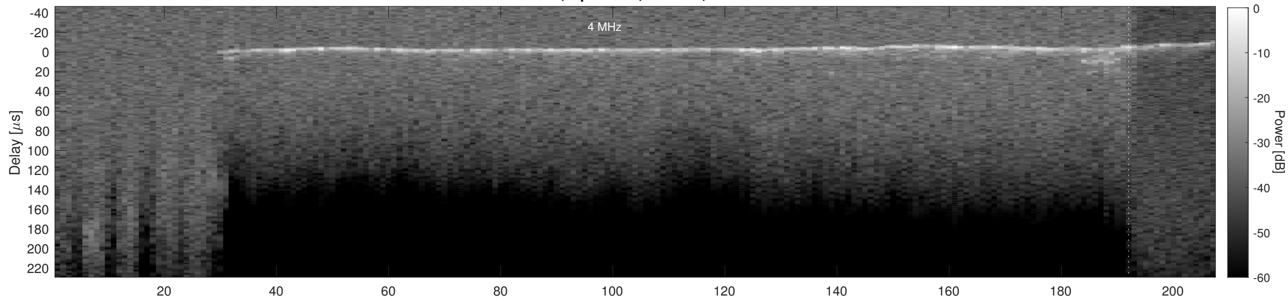
Orbit 3195, Cluttergram
