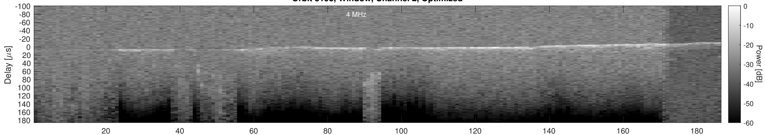
Orbit 3198, Cluttergram
