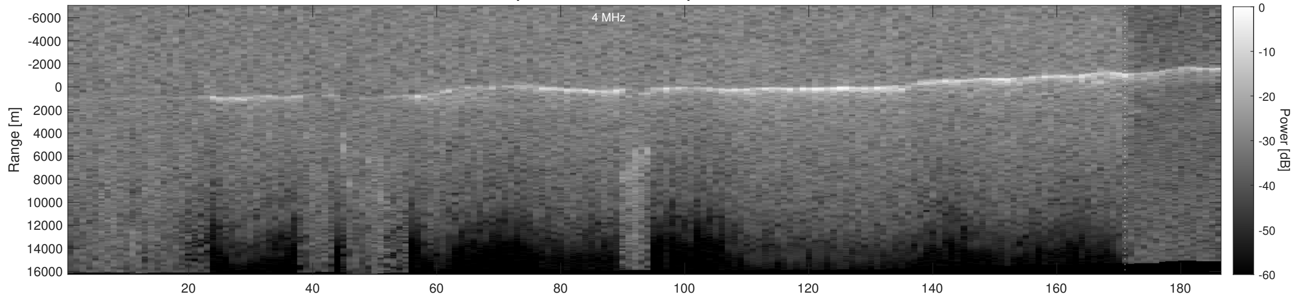
Orbit 3198, Depth-Corrected Cluttergram
