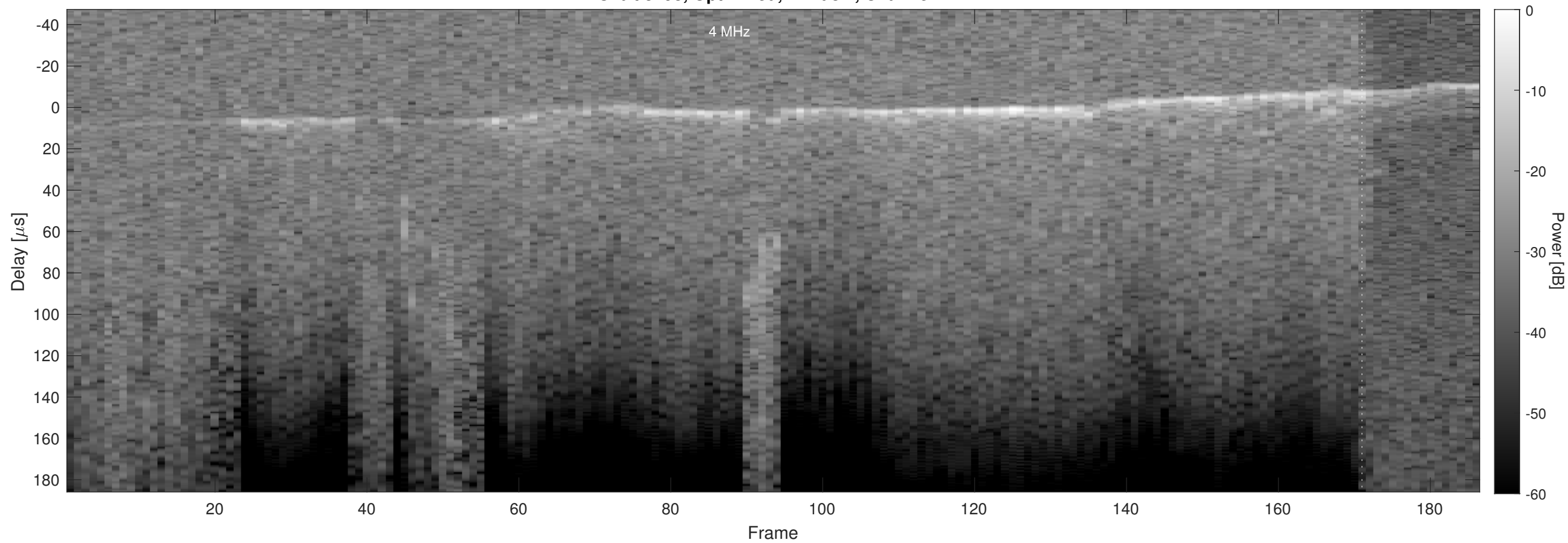
Orbit 3198, Optimized, Window, Channel 2
