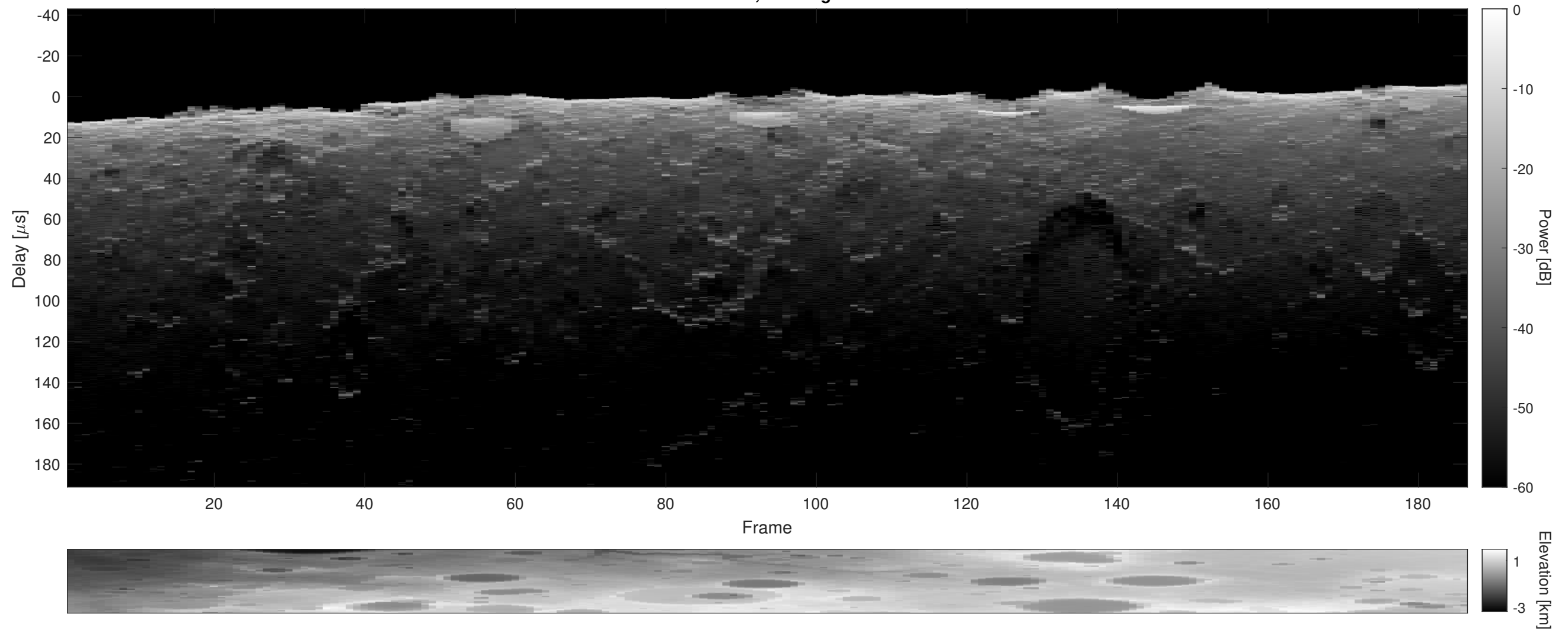
Orbit 3200, Cluttergram
