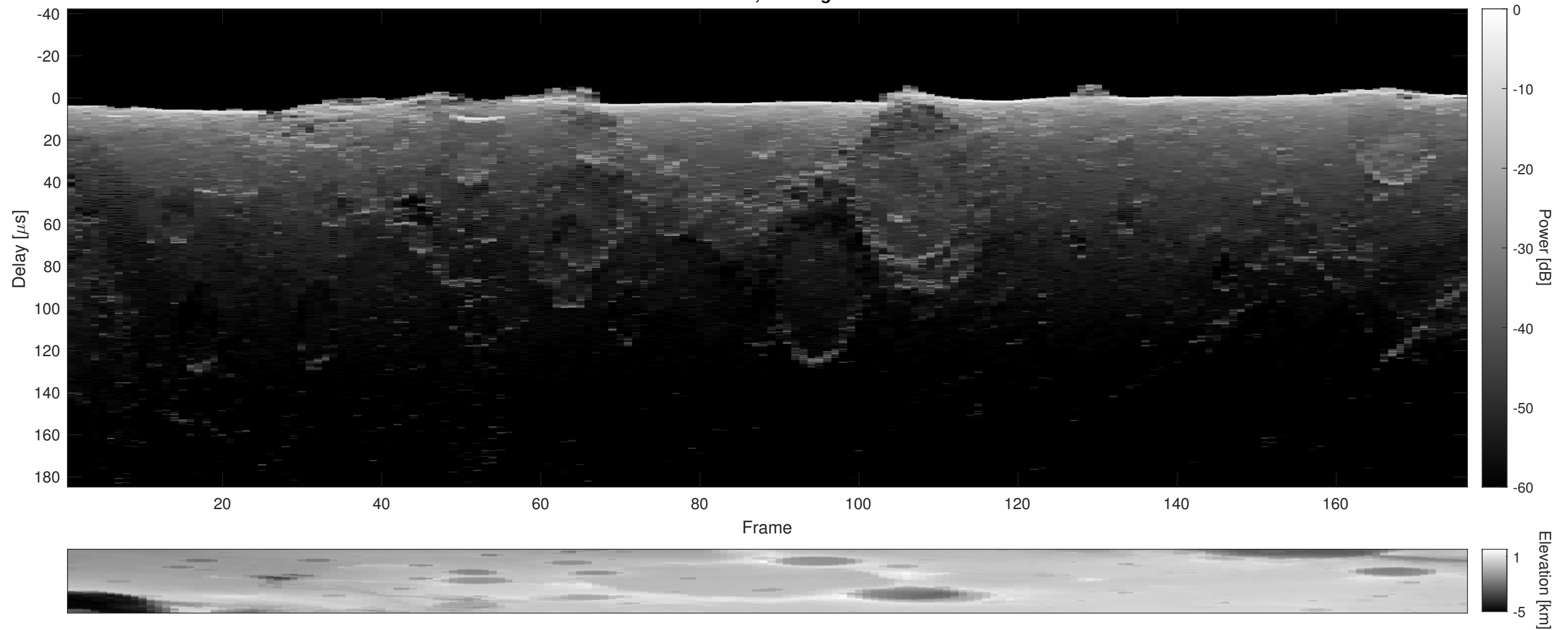
Orbit 3202, Cluttergram
