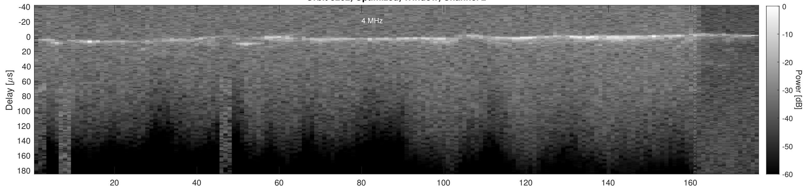
Orbit 3202, Cluttergram
