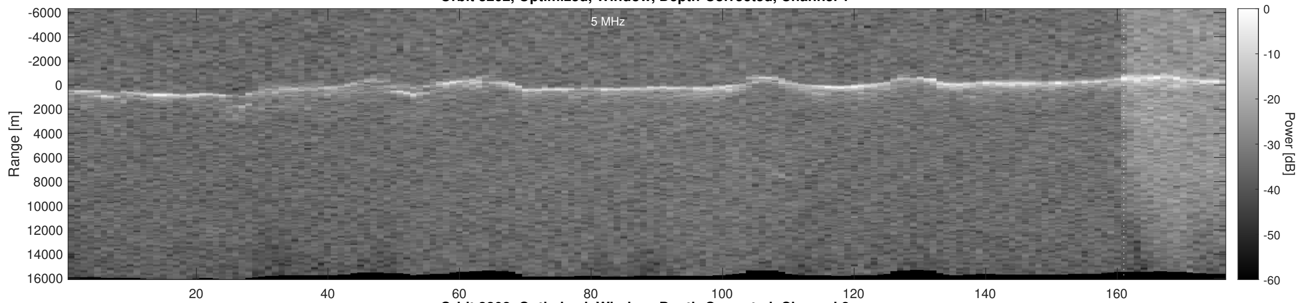
Orbit 3202, Optimized, Window, Depth-Corrected, Channel 2
