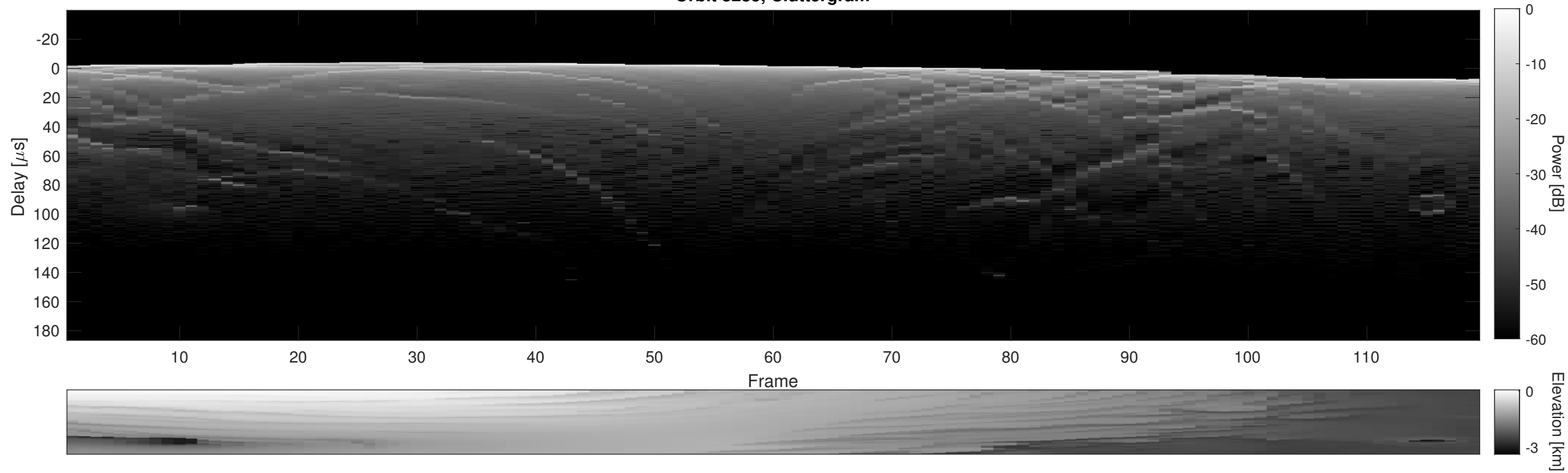
Orbit 3285, Cluttergram
