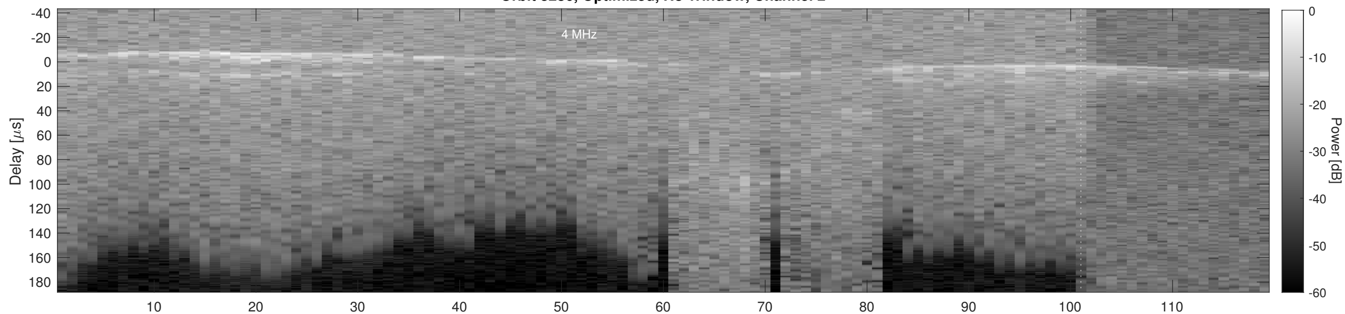
Orbit 3286, Cluttergram
