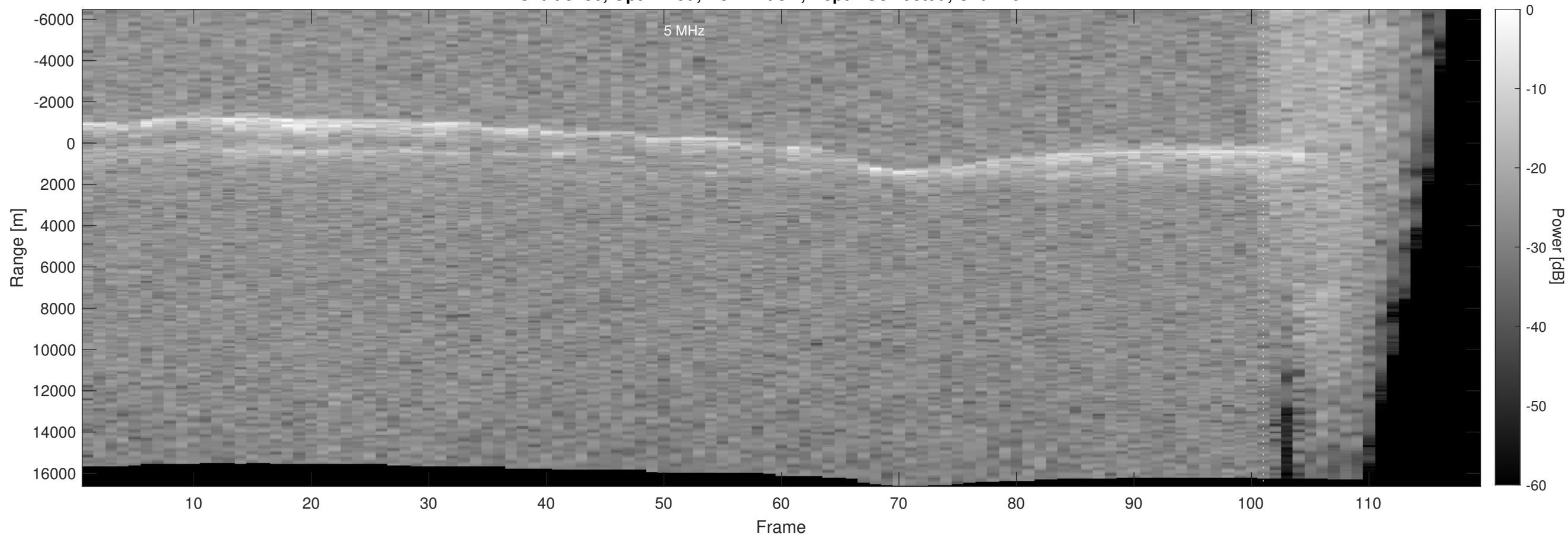
Orbit 3286, Optimized, No Window, Depth-Corrected, Channel 2
