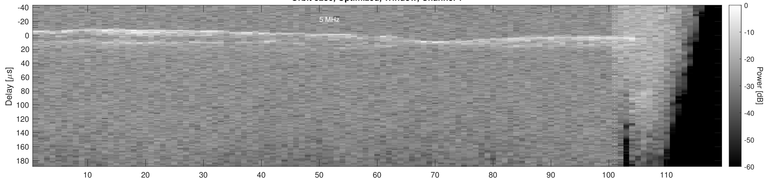
Orbit 3286, Optimized, Window, Channel 2
