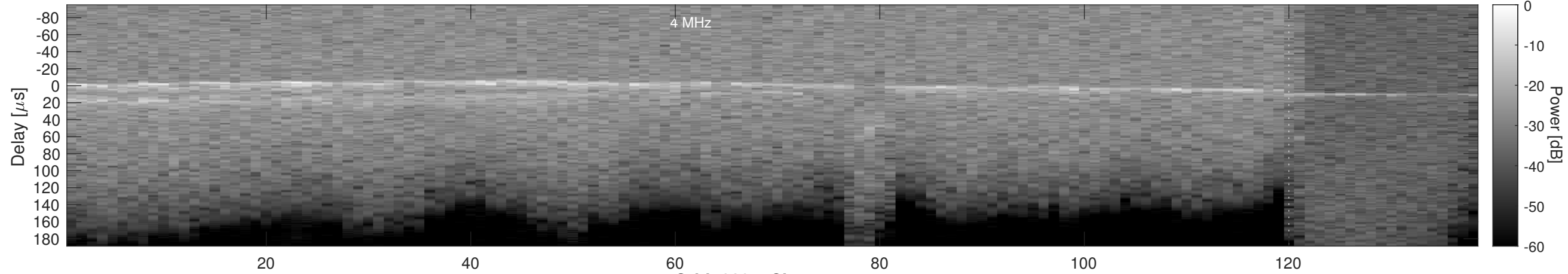
Orbit 3294, Cluttergram
