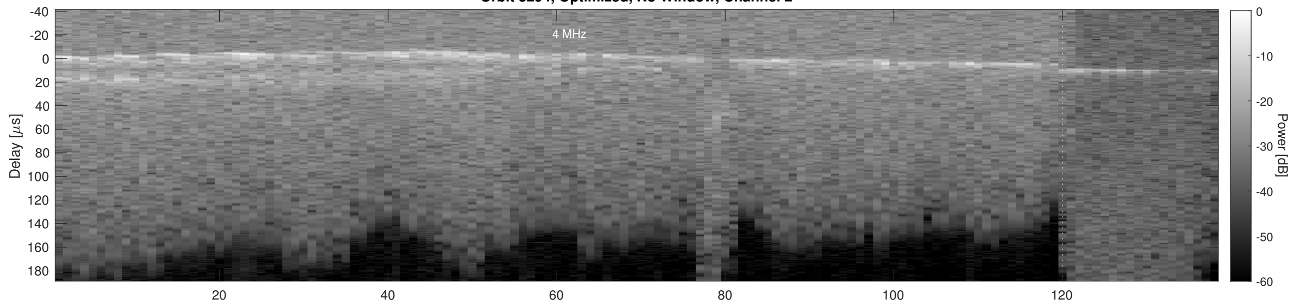
Orbit 3294, Cluttergram
