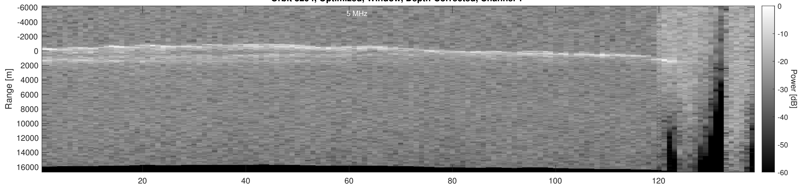
Orbit 3294, Optimized, Window, Depth-Corrected, Channel 2
