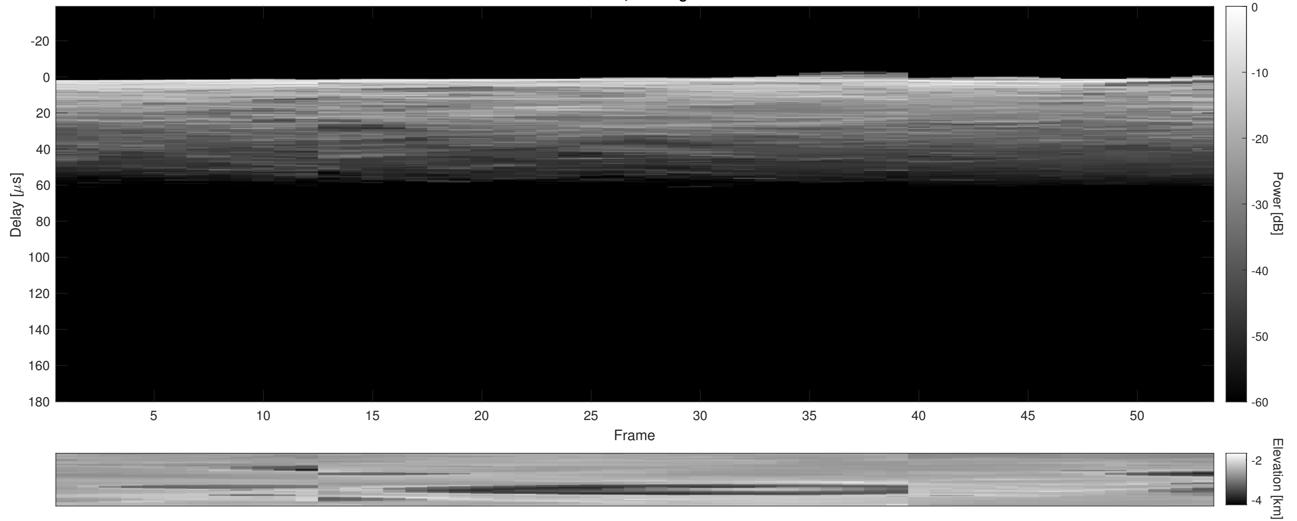
Orbit 3310, Cluttergram
