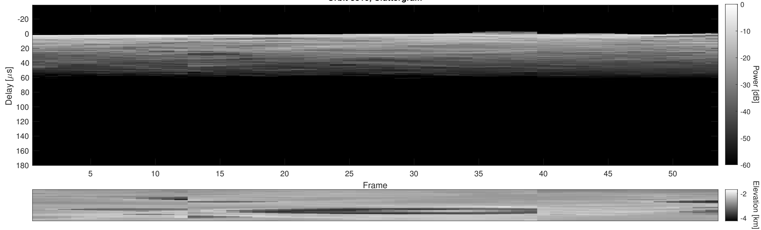
Orbit 3310, Cluttergram
