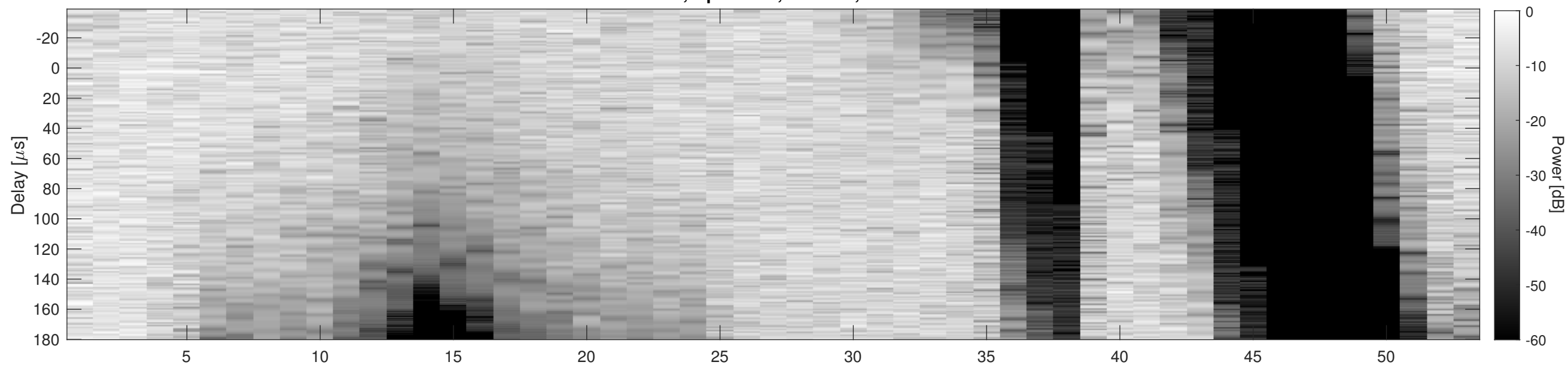
Orbit 3310, Cluttergram
