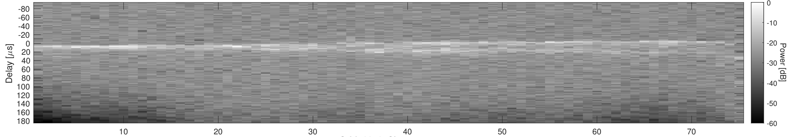
Orbit 3316, Cluttergram
