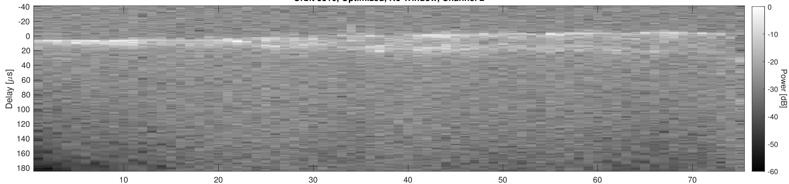
Orbit 3316, Cluttergram
