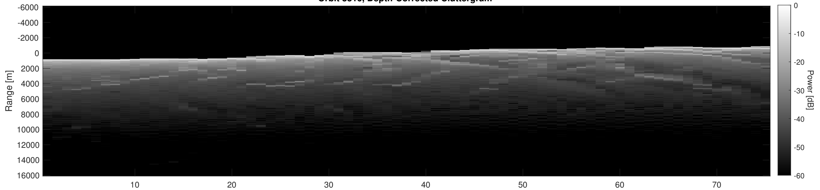
Orbit 3316, Depth-Corrected Cluttergram
