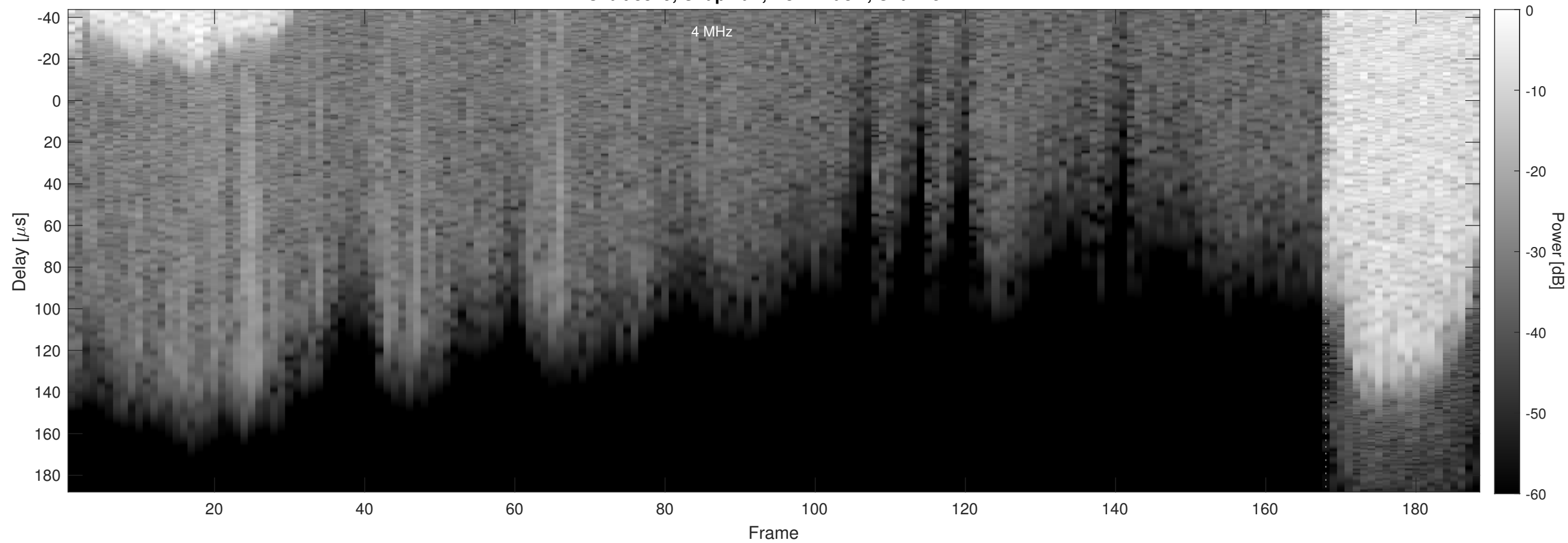
Orbit 3319, Chapman, No Window, Channel 2
