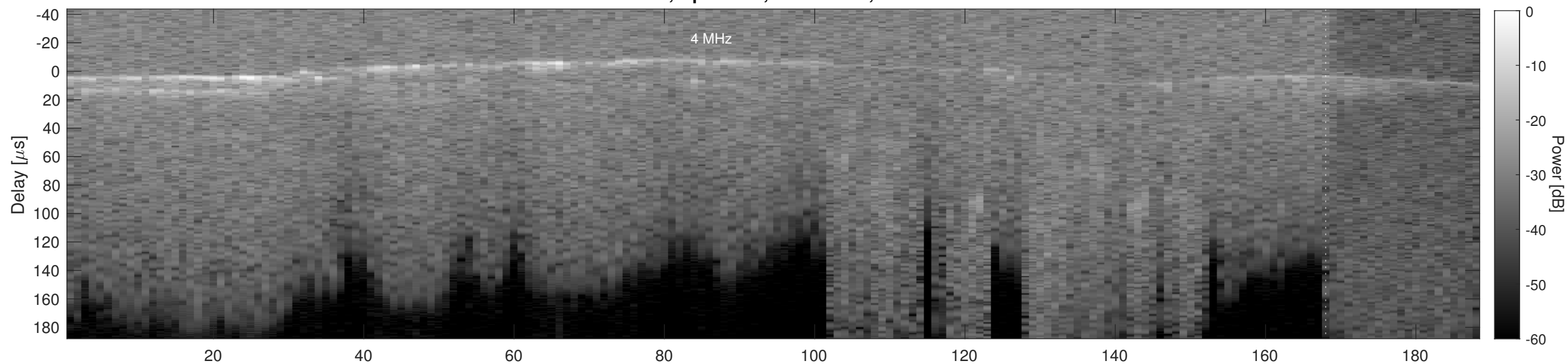
Orbit 3319, Cluttergram
