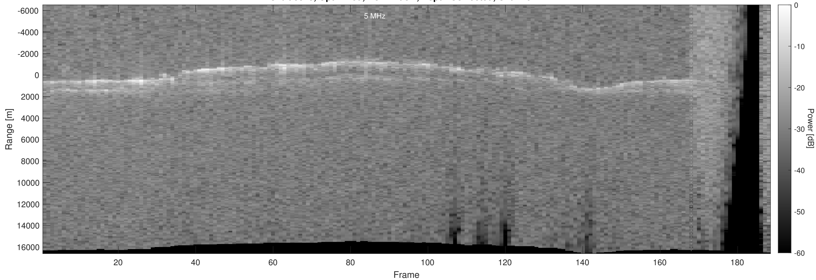
Orbit 3319, Optimized, No Window, Depth-Corrected, Channel 2
