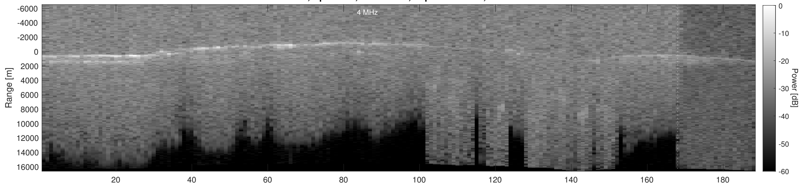
Orbit 3319, Depth-Corrected Cluttergram
