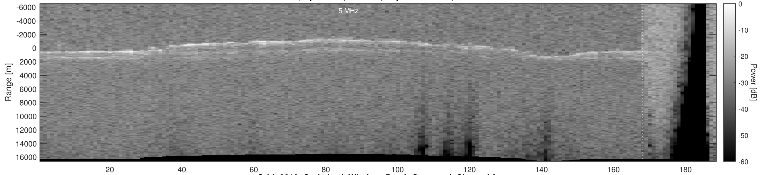
Orbit 3319, Optimized, Window, Depth-Corrected, Channel 2
