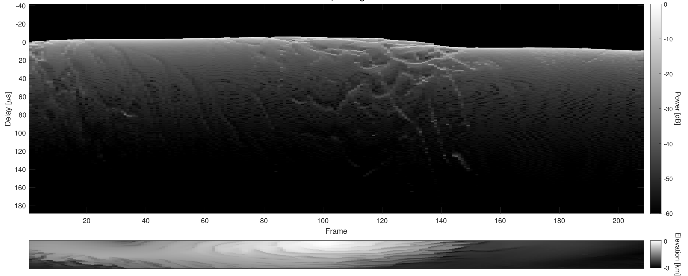
Orbit 3328, Cluttergram
