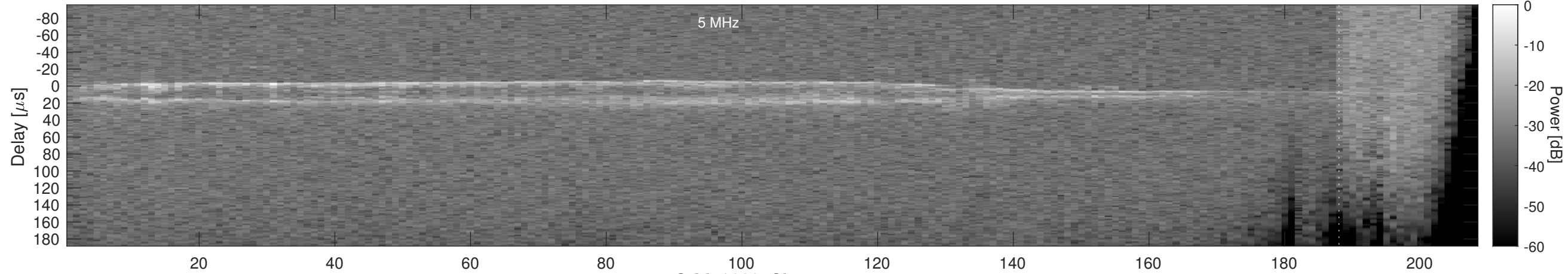
Orbit 3328, Cluttergram
