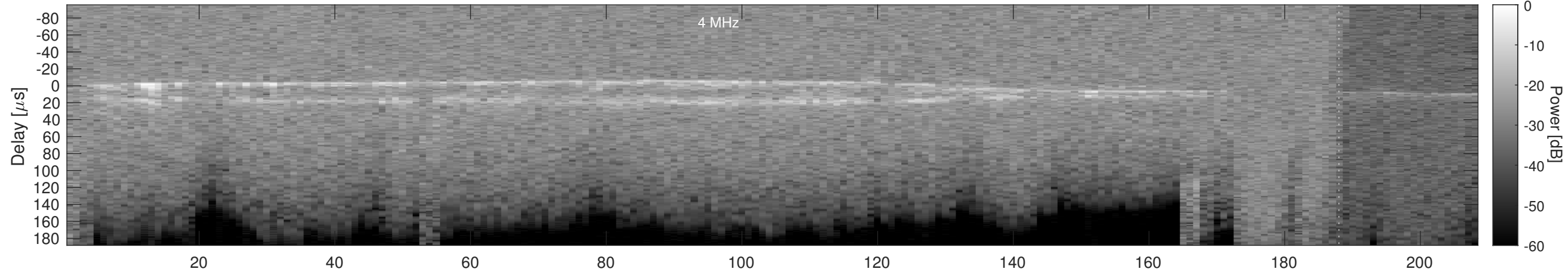
Orbit 3328, Cluttergram
