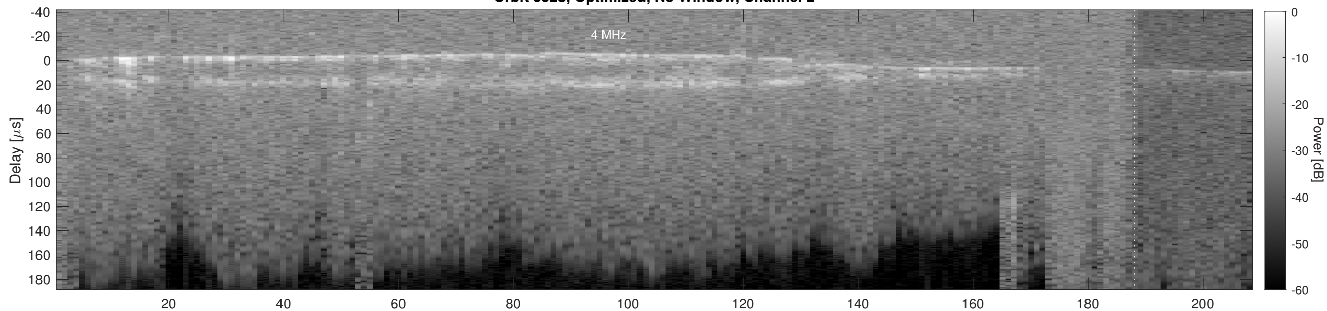
Orbit 3328, Cluttergram
