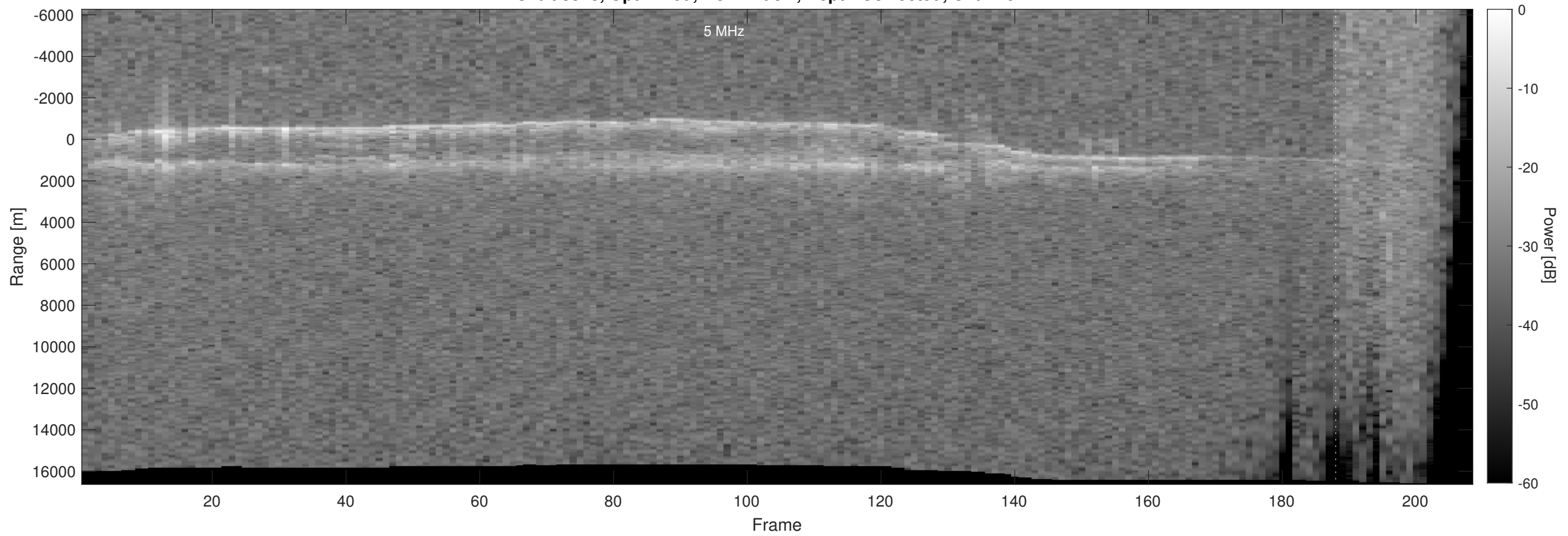
Orbit 3328, Optimized, No Window, Depth-Corrected, Channel 2
