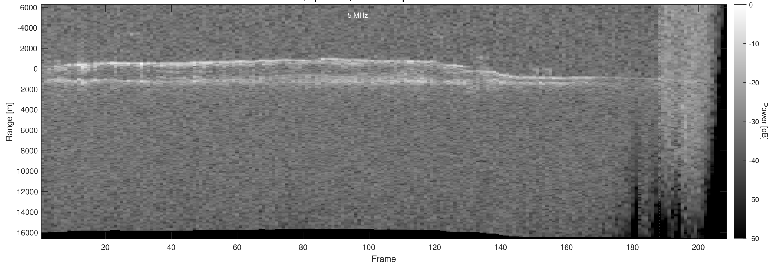
Orbit 3328, Optimized, Window, Depth-Corrected, Channel 2
