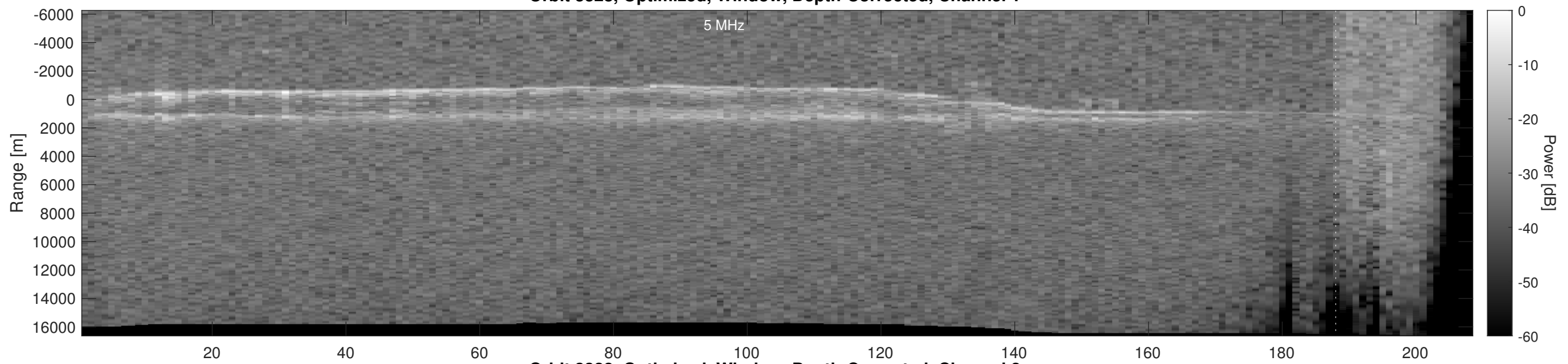
Orbit 3328, Optimized, Window, Depth-Corrected, Channel 2
