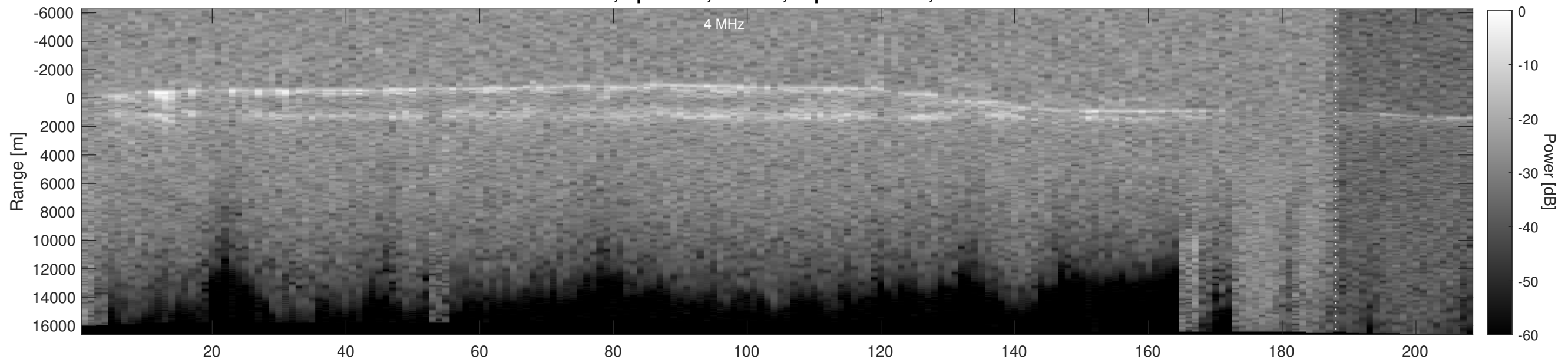
Orbit 3328, Depth-Corrected Cluttergram
