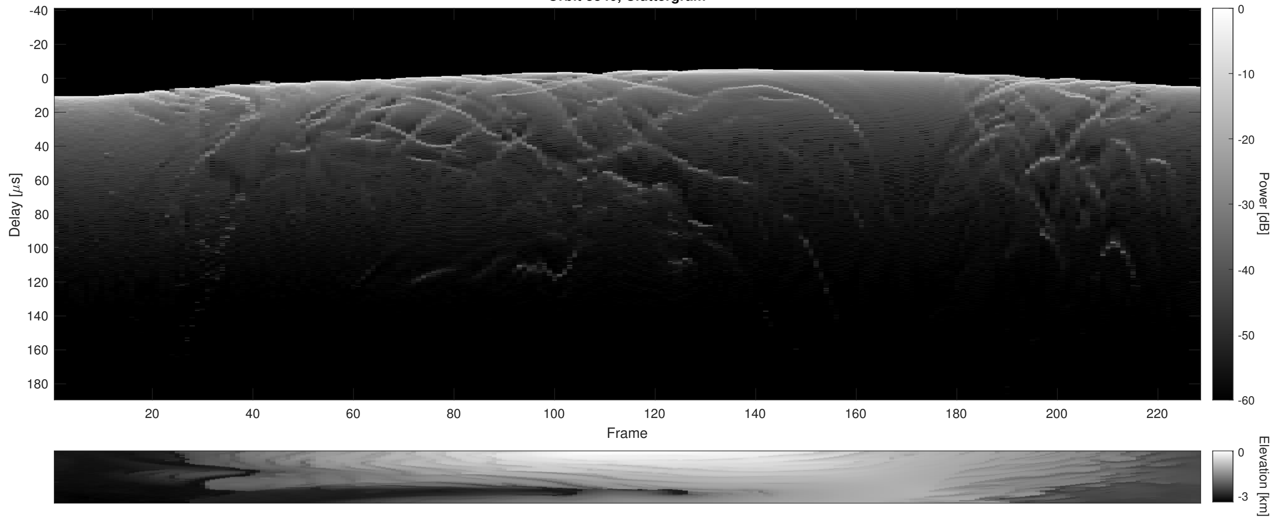
Orbit 3340, Cluttergram
