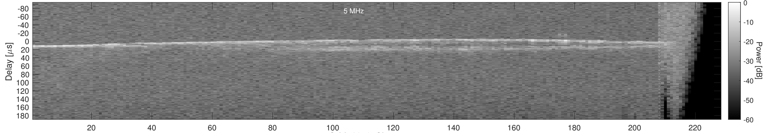
Orbit 3340, Cluttergram
