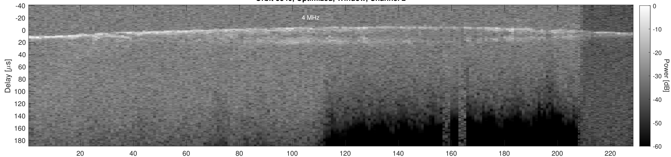
Orbit 3340, Cluttergram
