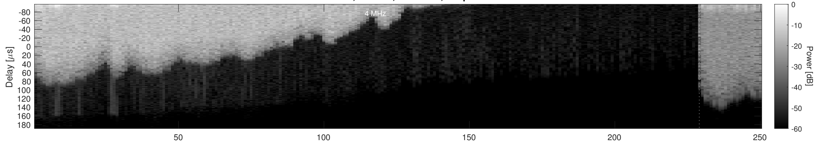
Orbit 3347, Window, Channel 2, Optimized
