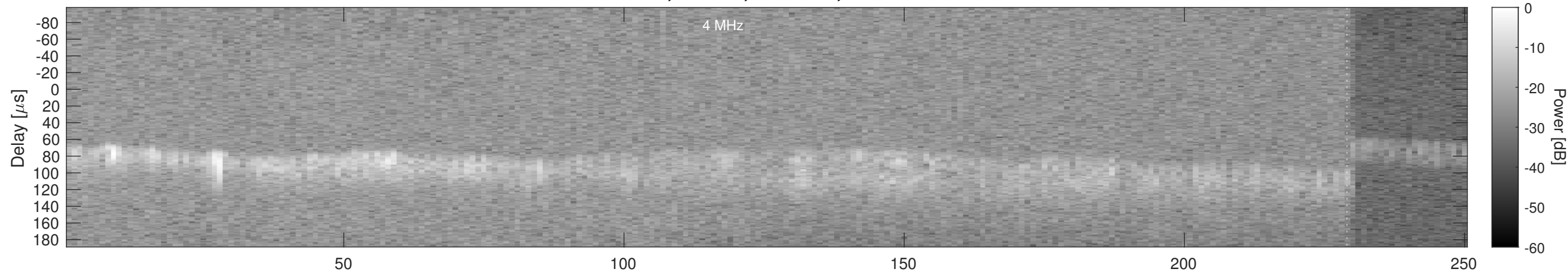
Orbit 3347, Window, Channel 2, Chapman
