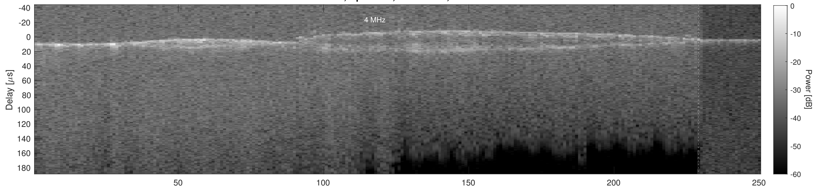
Orbit 3347, Cluttergram
