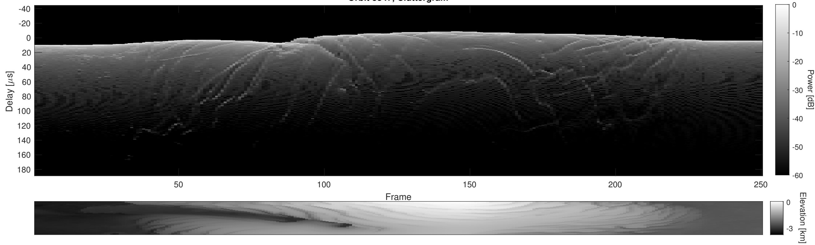
Orbit 3347, Cluttergram
