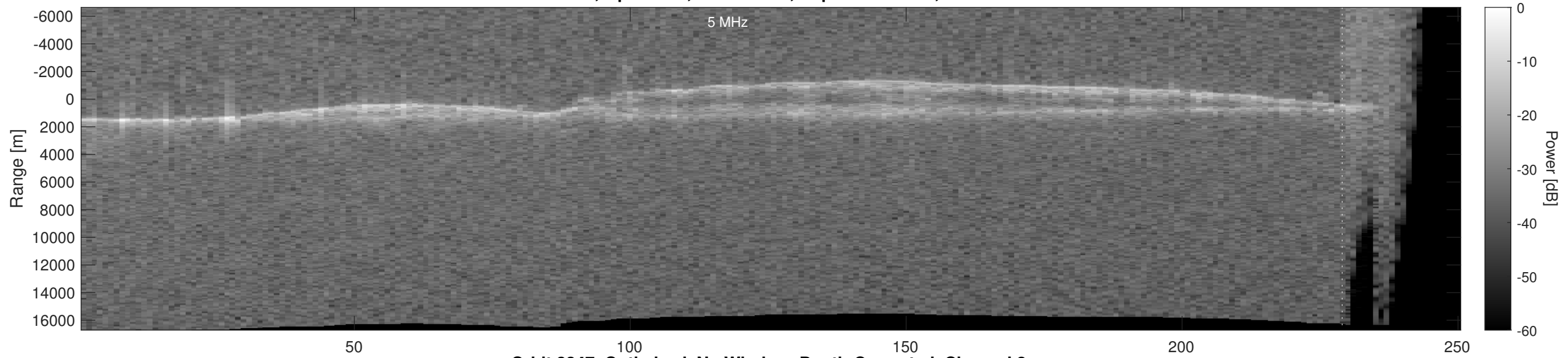
Orbit 3347, Optimized, No Window, Depth-Corrected, Channel 2
