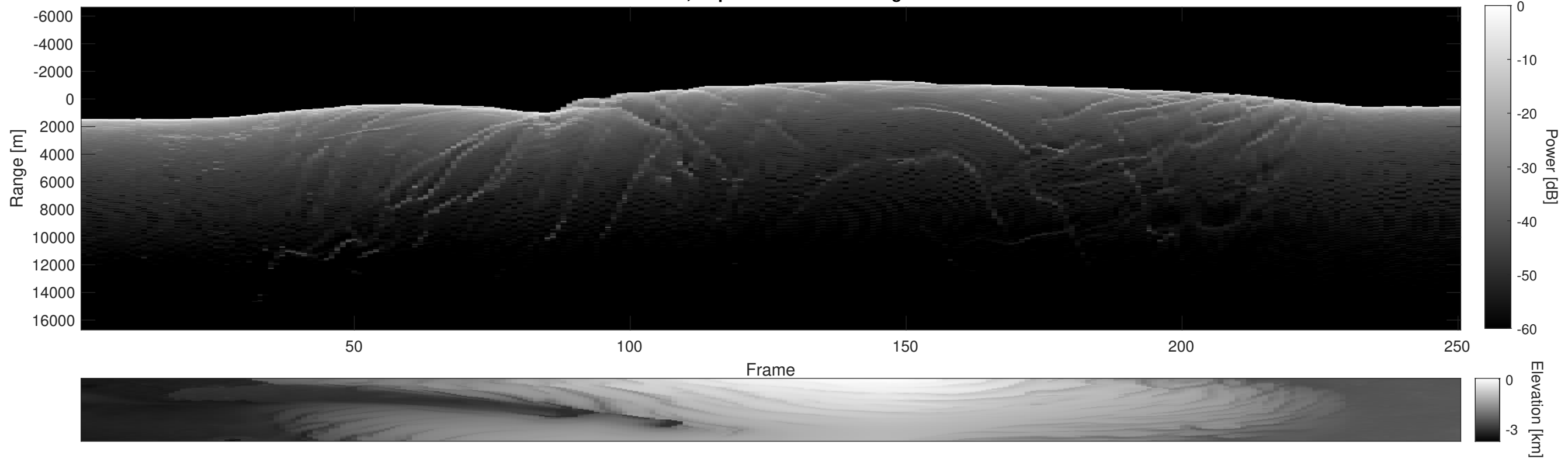
Orbit 3347, Depth-Corrected Cluttergram
