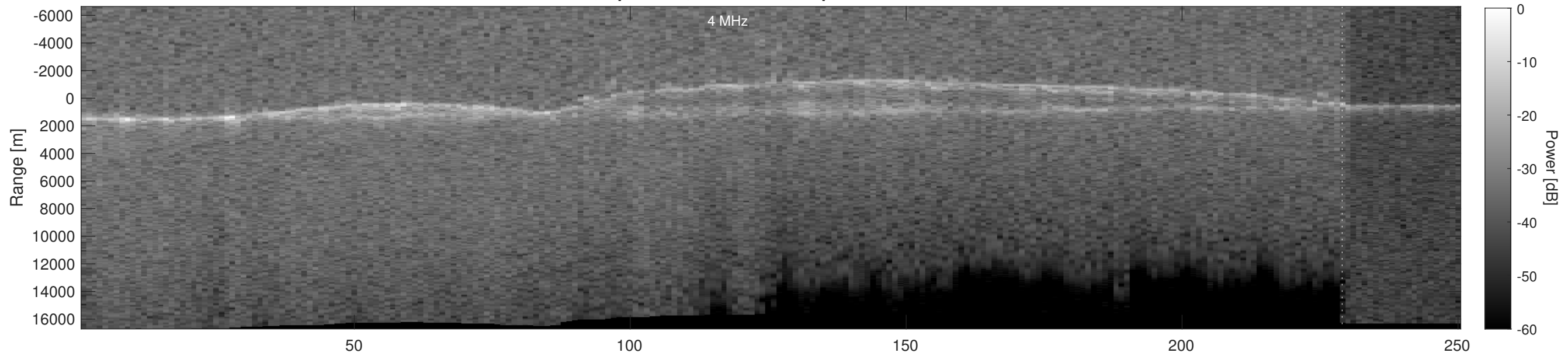
Orbit 3347, Depth-Corrected Cluttergram
