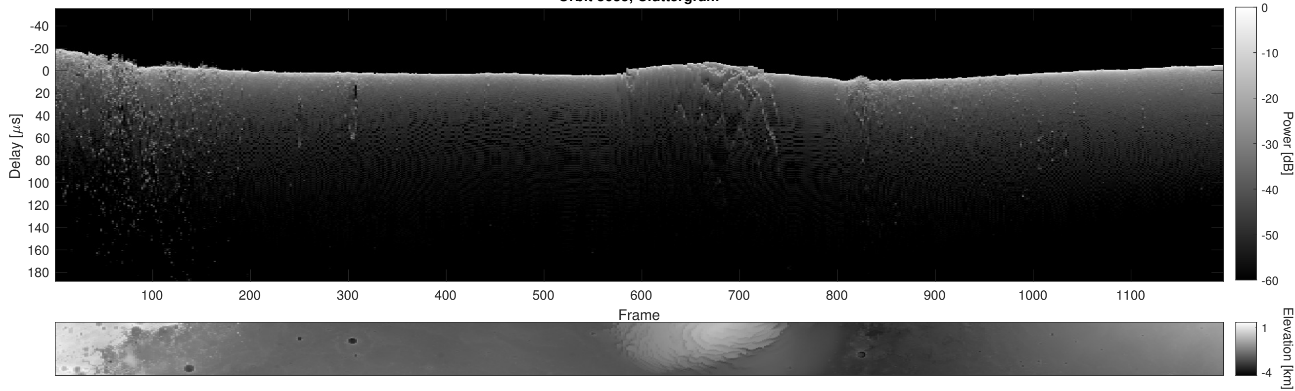
Orbit 3635, Cluttergram
