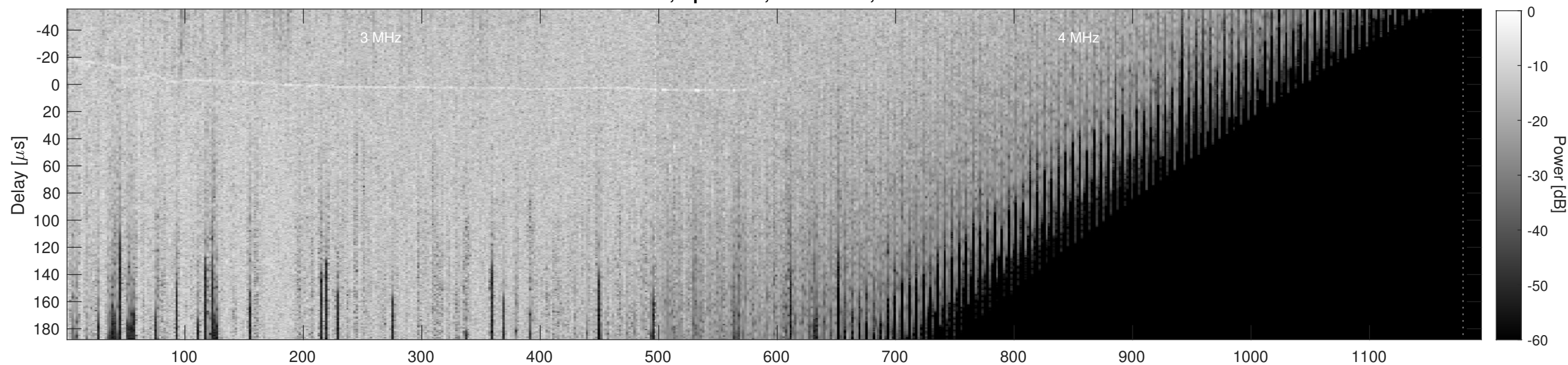
Orbit 3635, Cluttergram
