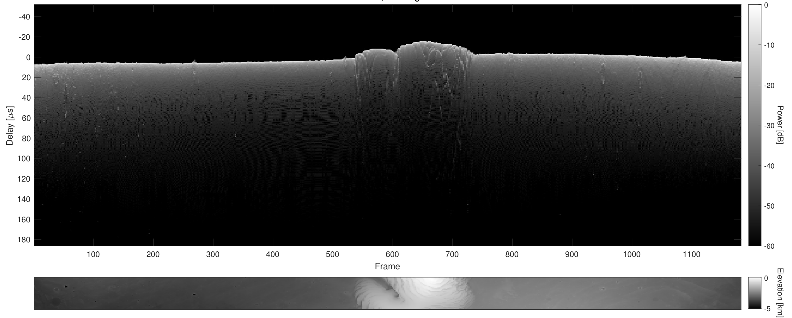
Orbit 3636, Cluttergram
