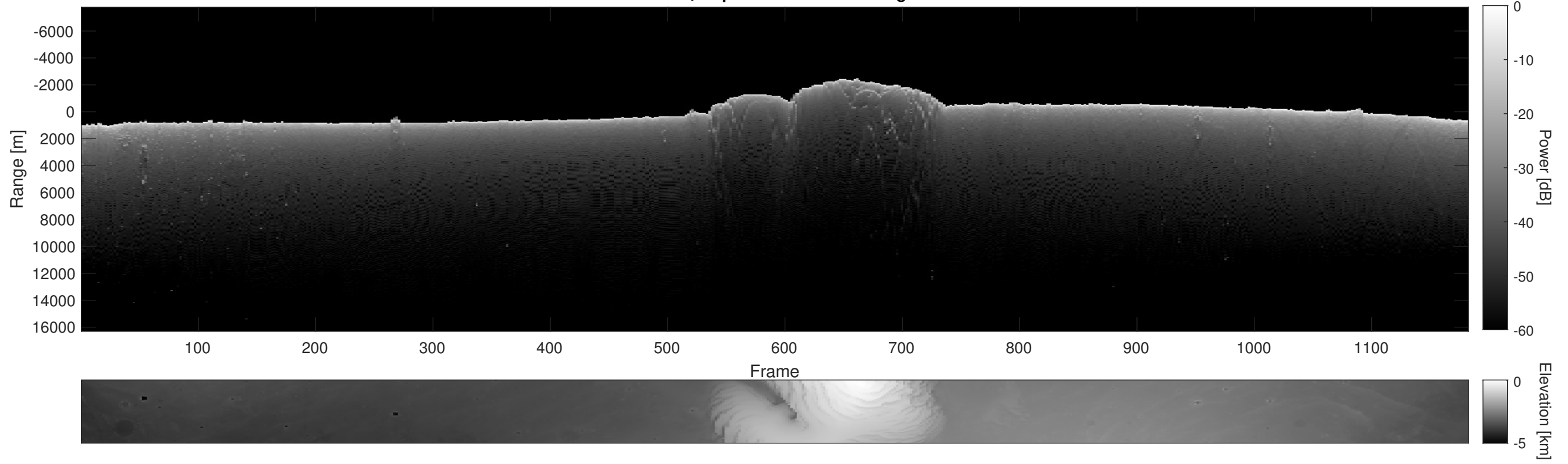
Orbit 3636, Depth-Corrected Cluttergram
