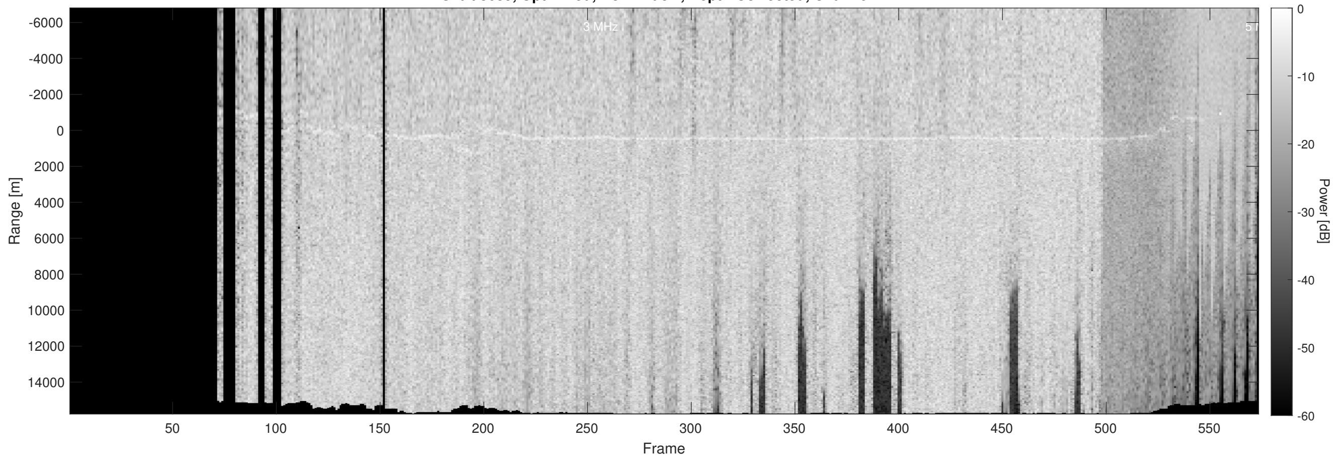
Orbit 3639, Optimized, No Window, Depth-Corrected, Channel 2
