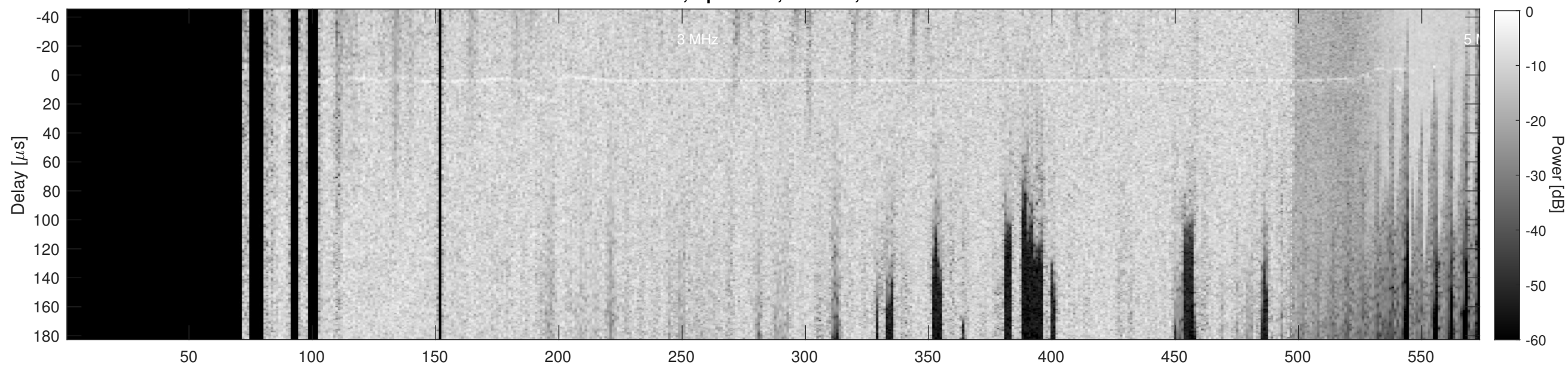
Orbit 3639, Cluttergram
