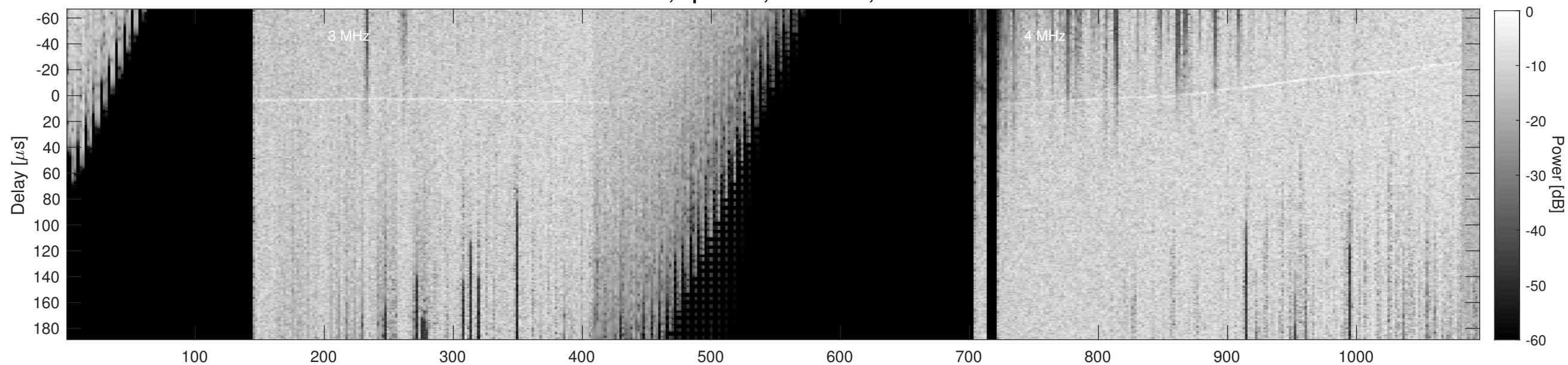
Orbit 3642, Cluttergram
