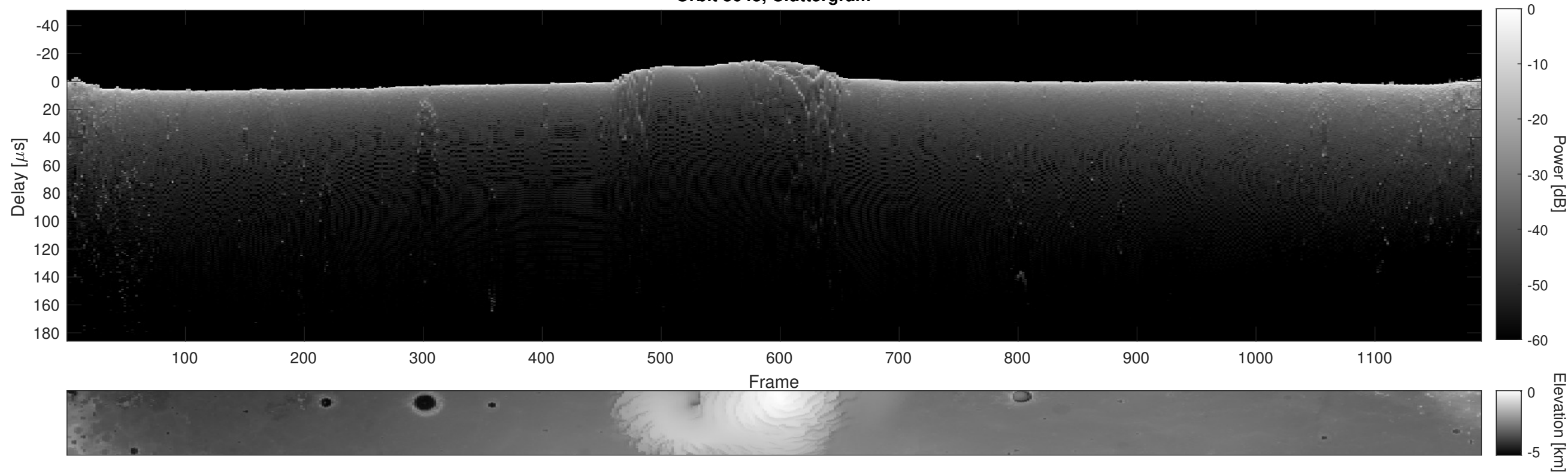
Orbit 3643, Cluttergram
