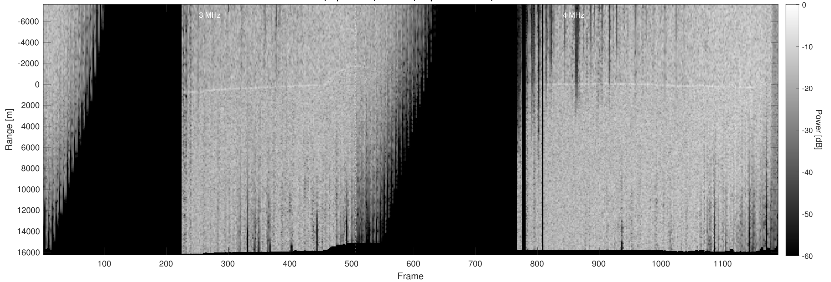
Orbit 3643, Optimized, Window, Depth-Corrected, Channel 2
